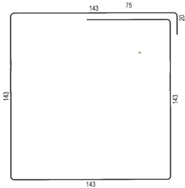
3 9ø12 L=6.67m
